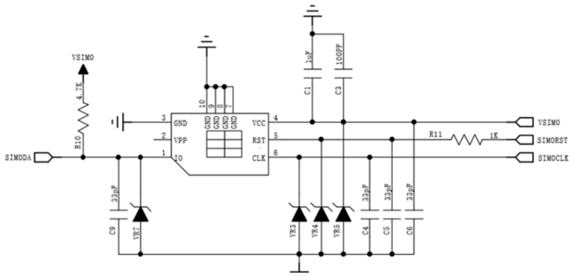
Figure 8. Using the 6PIN SIM Card Reference Circuit Diagram
